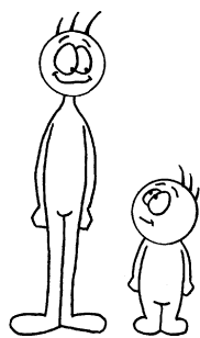
tall short
