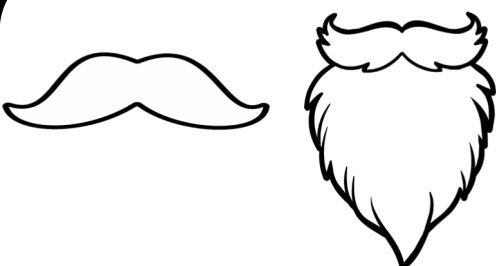
moustache beard
