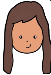
Long hair
